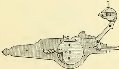
The German Wheel-lock.
